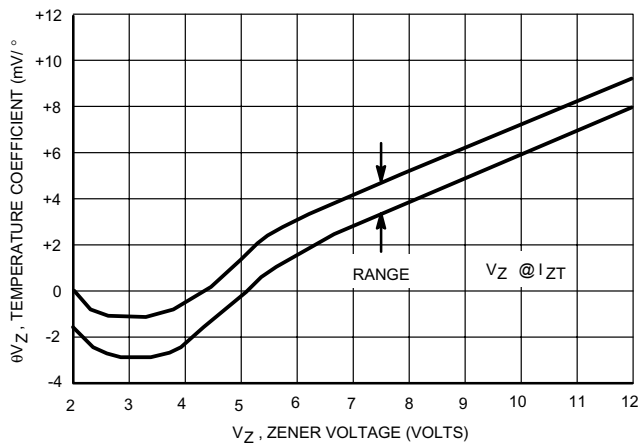
Figure 2. Temperature Coefficients
