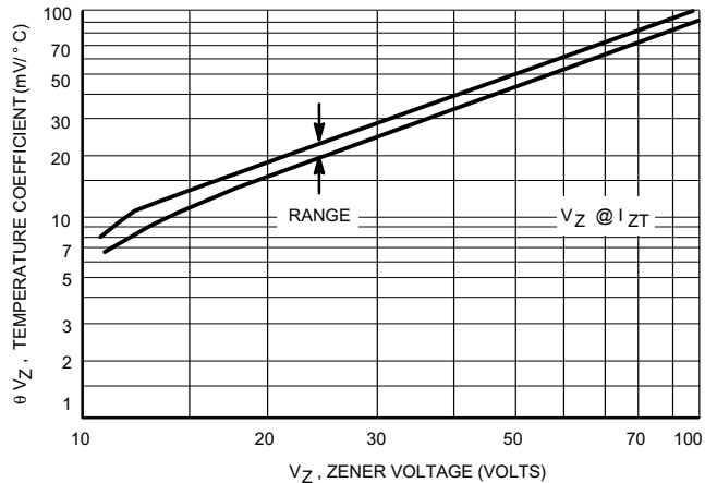
Figure 2. Temperature Coefficients
